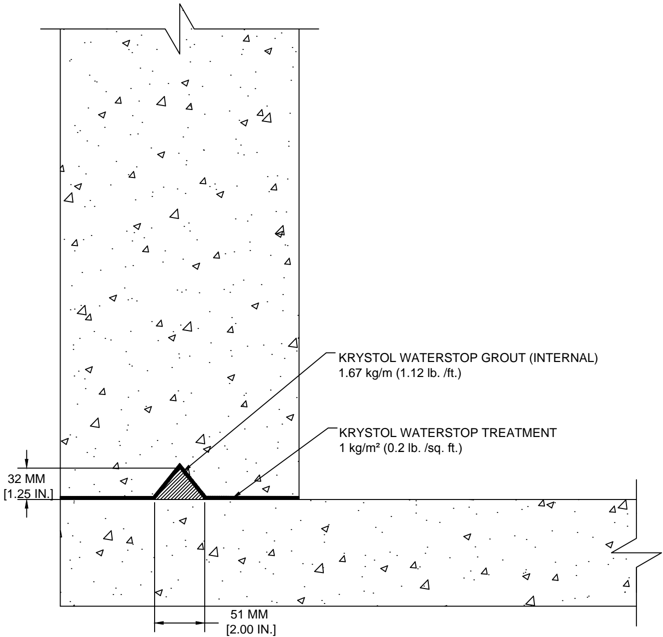
NEW CONSTRUCTION - WALL TO SLAB - SHOTCRETE (WALL ON TOP OF SLAB) REFER TO APPLICATION INSTRUCTION 4.21
