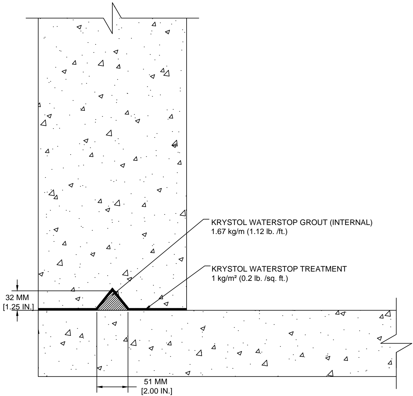
NEW CONSTRUCTION - WALL TO SLAB - (WALL ON TOP OF SLAB) REFER TO APPLICATION INSTRUCTION 4.11
